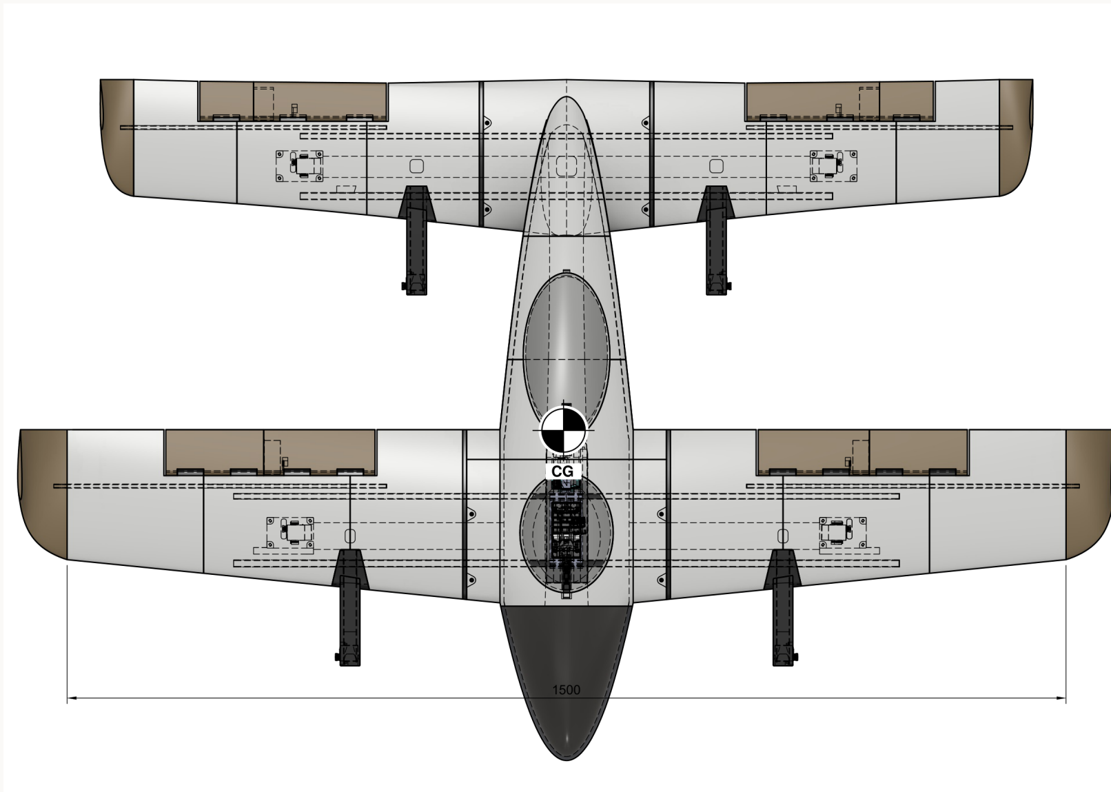
Top-view reference drawing with wing structure, motor positions, and CG marking.
